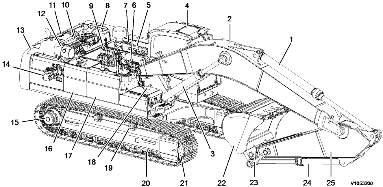
Figure 1 Component position
