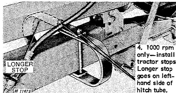
Hookup to Tractor-1000 rpm
