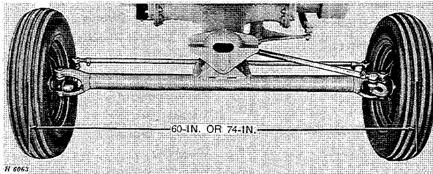
Wide-Tread Rear Axle
