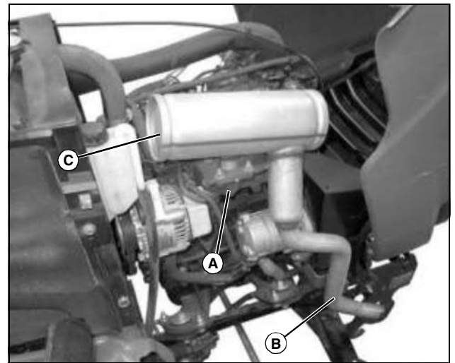
a. Exhaust manifold (A), muffler pipe (B), muffler (C) and muffer shield.
