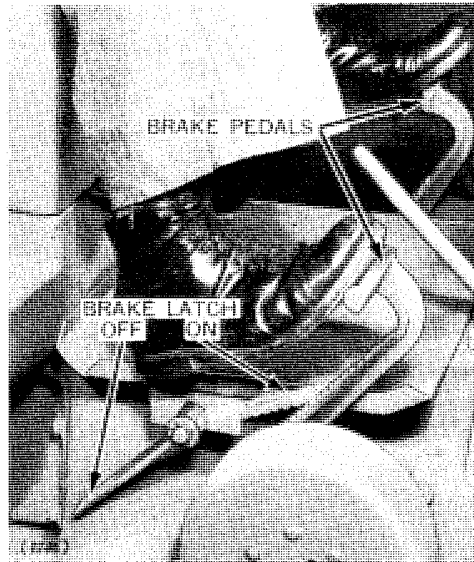
Brake Operation
