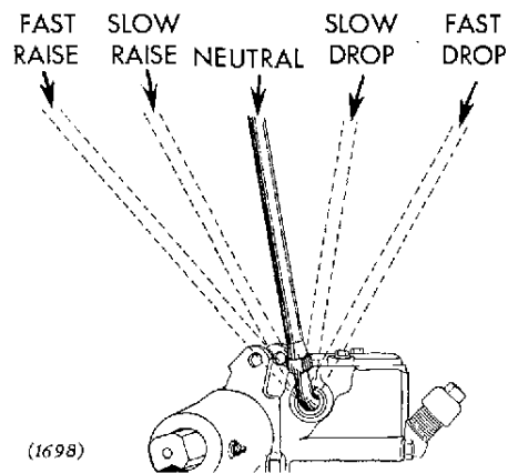
Powr-Trol Lever
