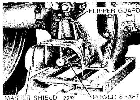
Power Shaft Flipper Guard
