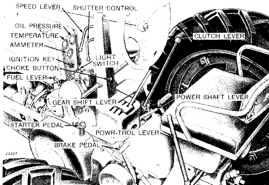
Controls of John Deere Model "B" Tractor
