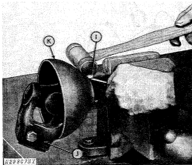
I—Locking Bearing J—Yoke and Tube Assembly K—Rear Shield
