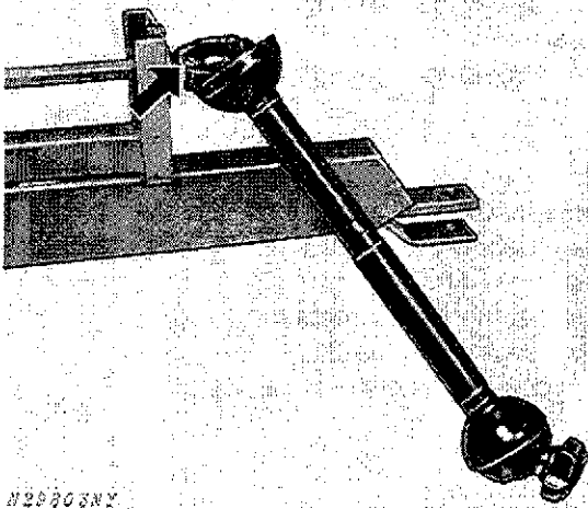
Fig. 2-Removing Powershaft
