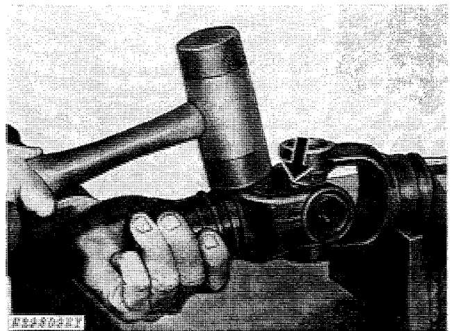
Fig. 8-Removing Spider and Bearing Assembly
