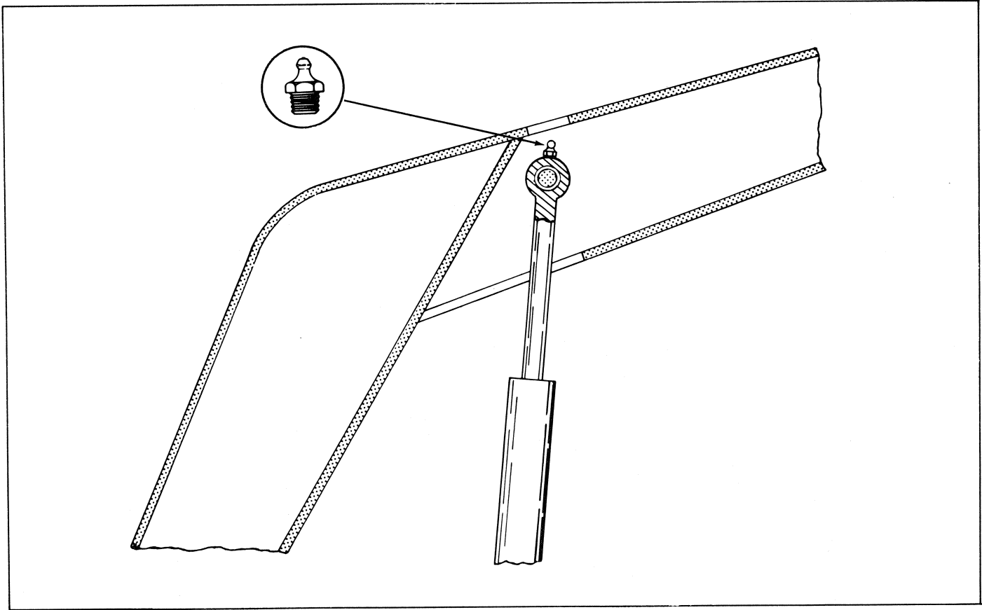
Figure 12. Grease Fitting on Rod End of Hoist Cylinder. Access through Hole in top of Beam.
