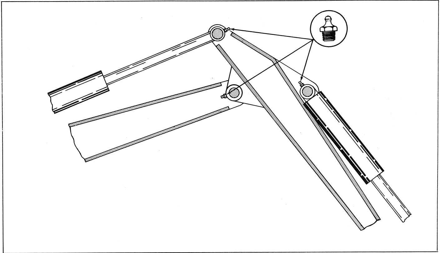
Figure 14. Grease Fitting on Base End of Tool Cylinder, Rod End of Crowd Cylinder and Intermediate to Dipperstick Hinge Pin.
