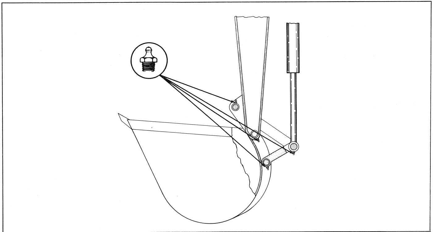
Figure 15. Grease Fittings on Rod End of Tool Cylinder, Dipperstick to Bucket Hinge Pin and Connecting Link Hinge Pins.
