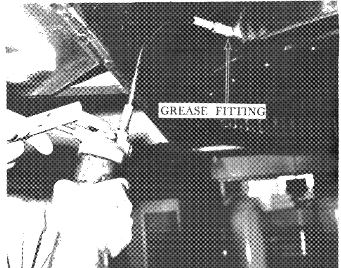
Figure 2. Grease Fitting Turntable Bearing (one of four)
