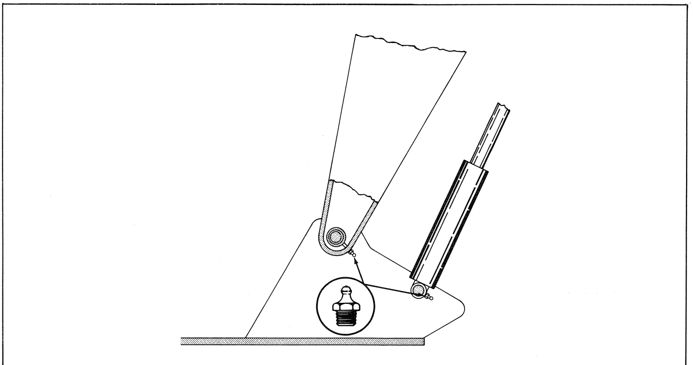
Figure 11. Grease Fittings on Base End of Hoist Cylinder and Main Boom to Mast Hinge Pin.
