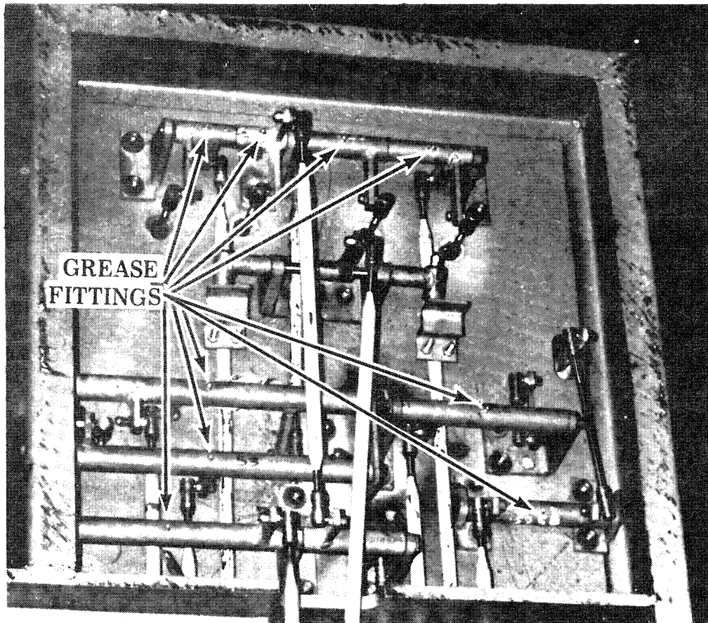
Figure 8. Grease Fittings on Bellcranks Under Operator's Cab.
