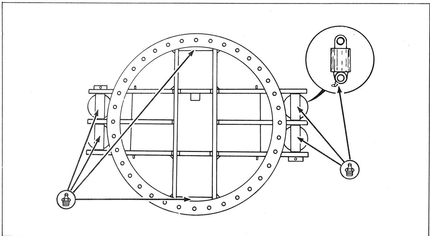
Figure 9. Leveler Grease Fitting Locations.
