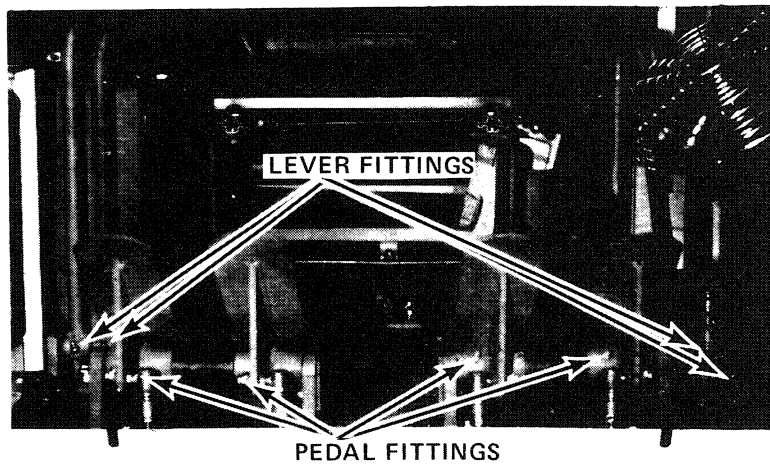
Figure 6. Grease Fitting on Pedal and Lever Linkage
