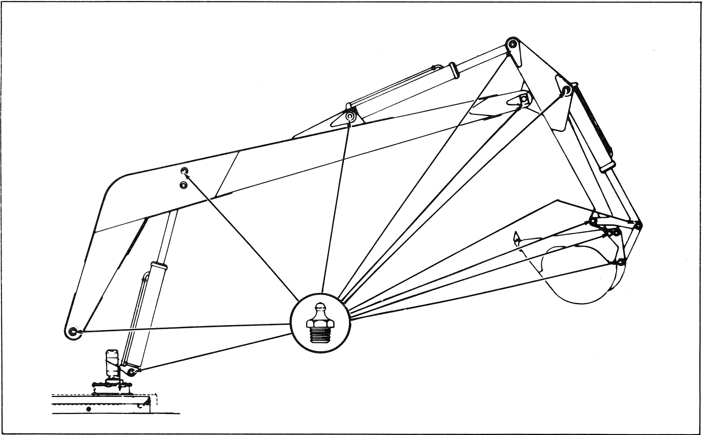
Figure 10. Boom and Cylinders Grease Fittings
