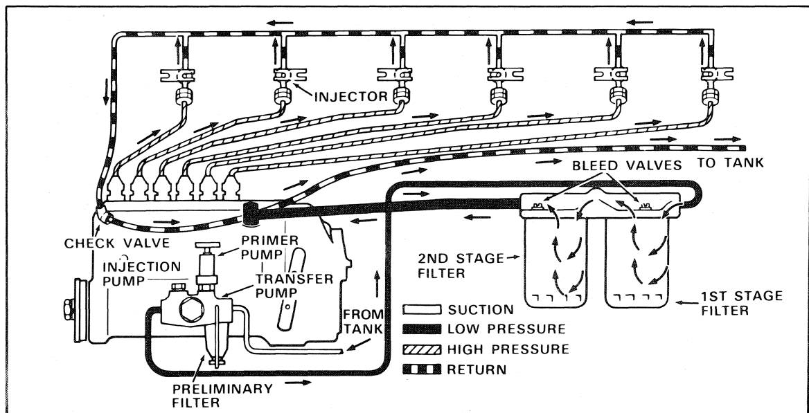
Figure 18. Fuel Flow and Return to Tank
