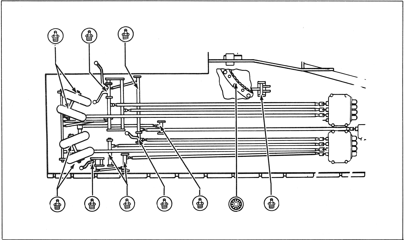
Figure 4. Control Linkage and Bellcrank Grease Fittings.
