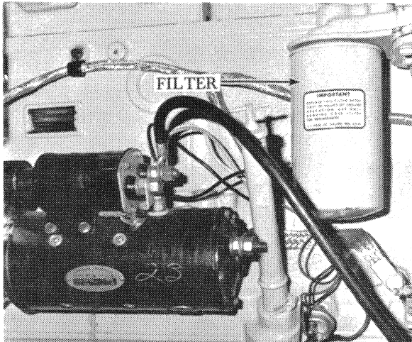
Figure 17. Engine Oil Filters
