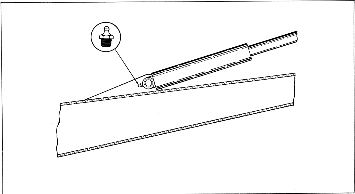
Figure 13. Grease Fitting on Base End of Crowd Cylinder
