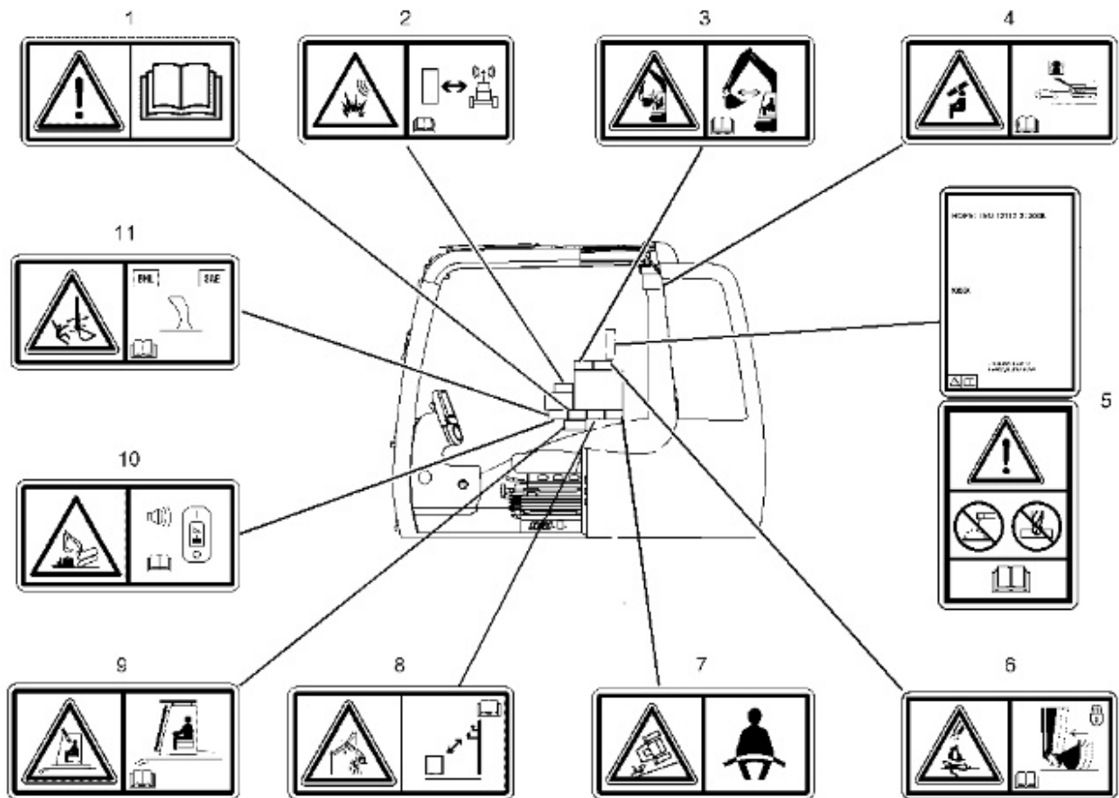
Illustration 1 View of the cab
