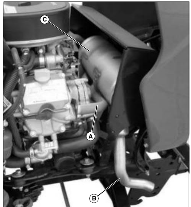
a. Exhaust manifold (A), muffler pipe (B), muffler (C) and muffler shield.
