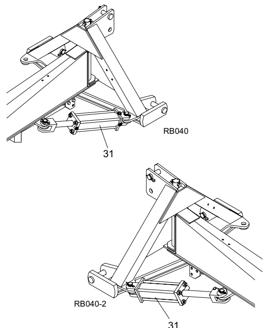
Figure 6. Hydraulic Offset
