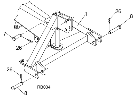
Figure 1. 3-point Hitch Connection
