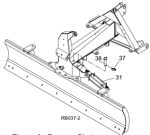
Figure 3. Reverse Blade
