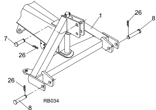
Figure 1. 3-point Hitch Connection
