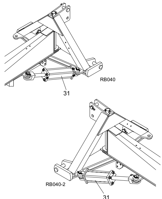
Figure 6. Hydraulic Offset
