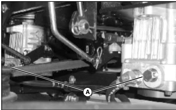
A - Free-Wheeling Pump Release Valves
