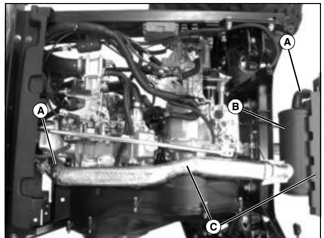
a. Muffler pipes (A), muffler (B), and muffler shields (C).
