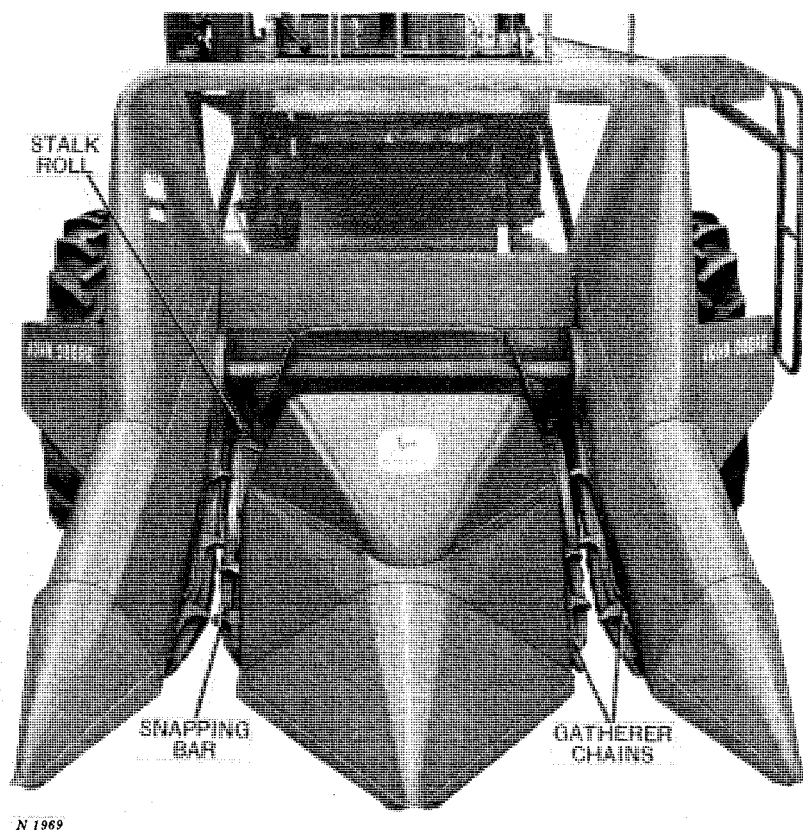
John Deere 205 Corn Attachment on 40 Self-Propelled Combine
