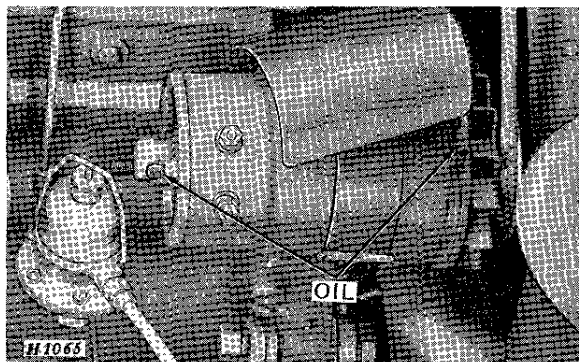
Generator
