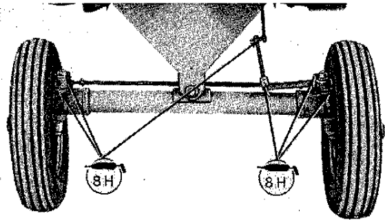
CONVENTIONAL STEERING
