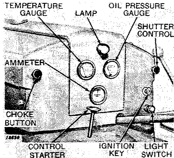
Instrument Panel
