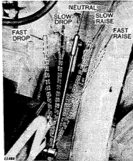
Powr-Trol Lever
