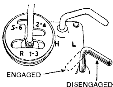
Power Shaft Shift Lever in Disengaged Position
