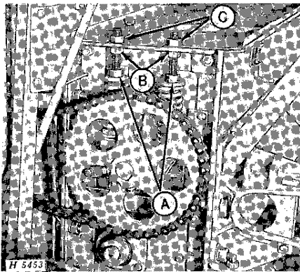
Roller Spacing and Pressure Adjustments
