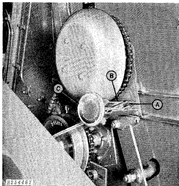
A—Pointer B—RPM Indicator C—Fan Speed Control Wheel
