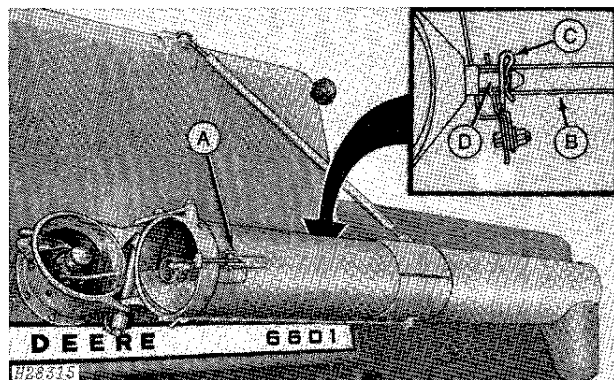
A—Over-Center Lock B—Transport Support C—Spring Pin D—Locking Stud
