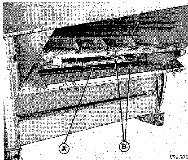
A—Sieve Opening Control Lever B—Chaffer Opening Control Lever
