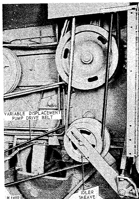
Hydraulic Propulsion Drive on 105 Combine
