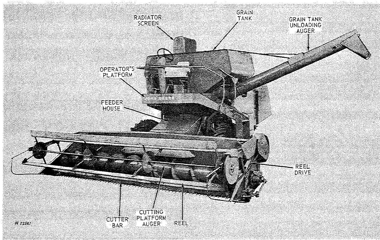
John Deere 95 Combine
