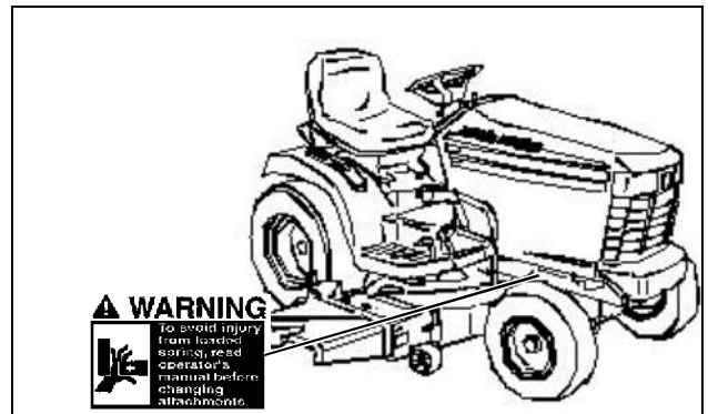
MX30477, M146577
