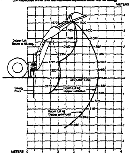
410B BACKHOE LIFT PER SAE J31 (Lift capacities are 67% of the maximum anywhere within the full swing)
