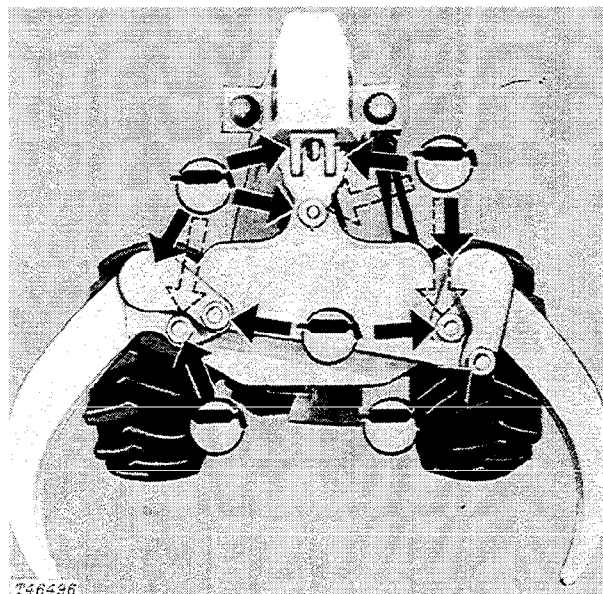
Fig. 15-Grapple Pins (12 points)
