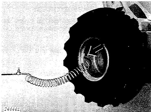
Fig. 4-Correct Tire Filling Procedure
