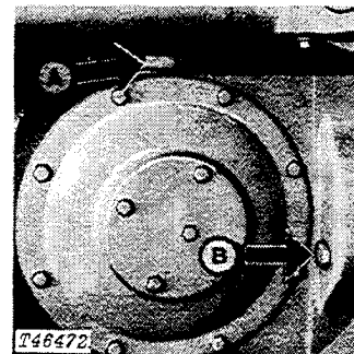
A—Filler Plug B—Oil Level Plug
