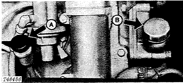
A—Dipstick B—Oil Filler Cap
